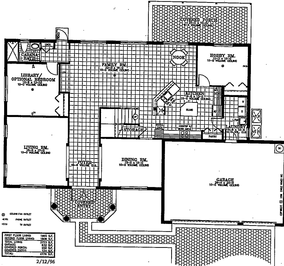
FIRST FLOOR
